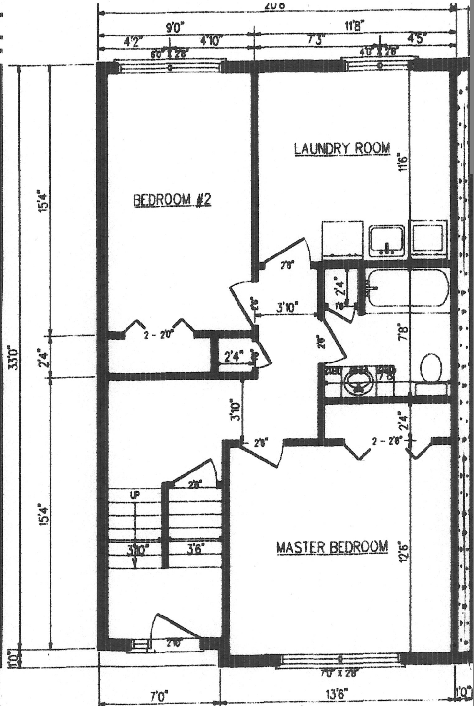
KENTVILLE SEMI-DETACHED HOME MAIN FLOOR LEVEL 21' X 34' X 33' KENTVILLE SEMI-DETACHED HOME BASEMENT LEVEL
