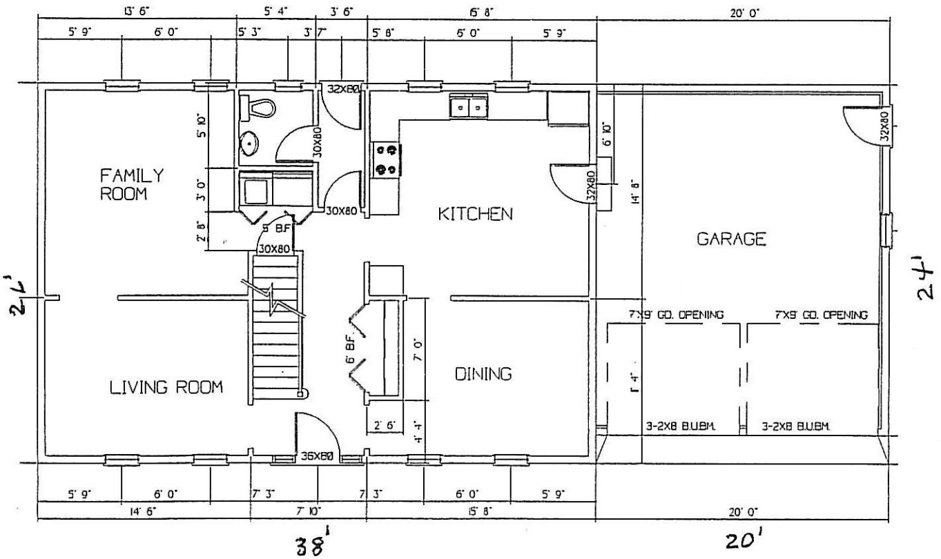
THE WOLFVILLE 38 X 26 (GARAGE 20 X 24)
